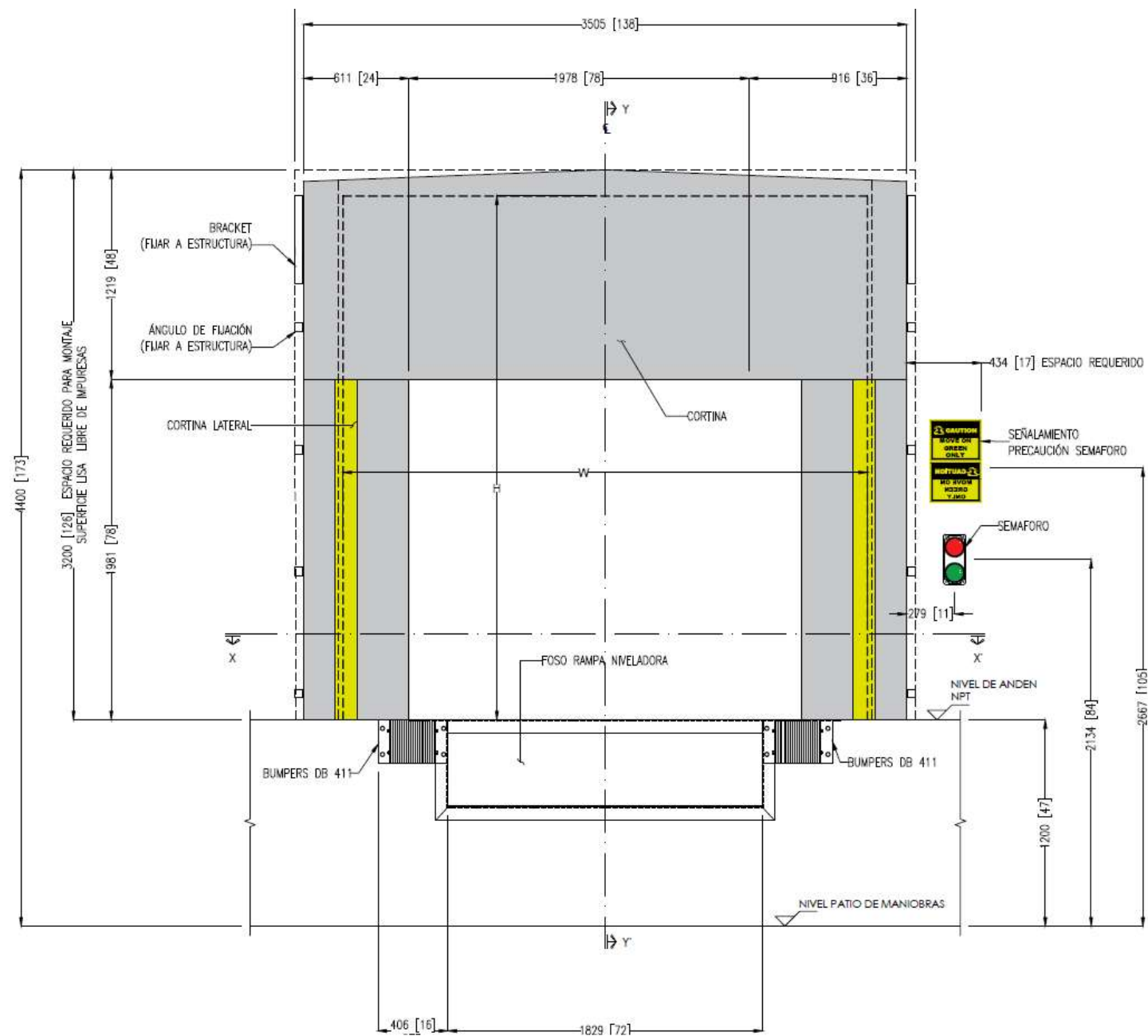
VISTA FRONTAL EXTERIOR
